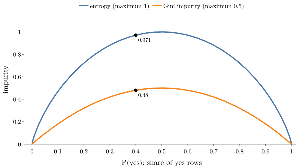
Figure 8: Entropy and Gini impurity against the share of yes observations
