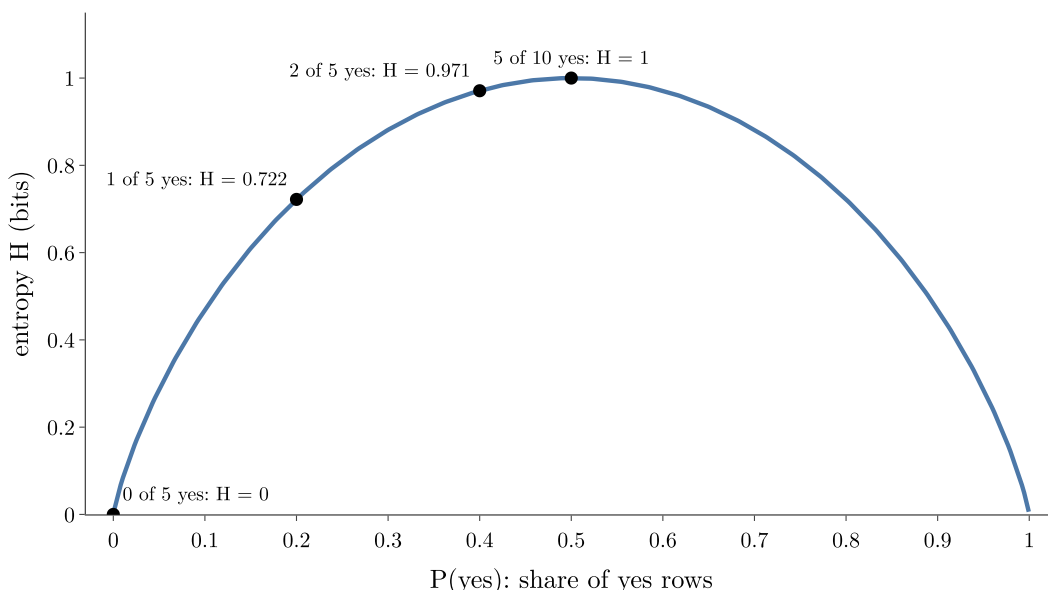
Figure 5: Two-class entropy against the share of yes observations
