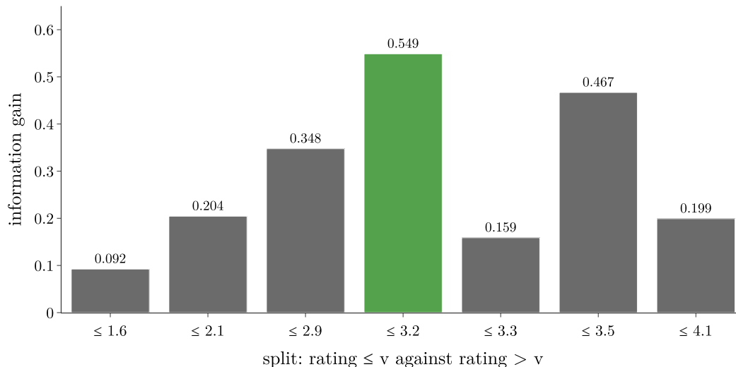
Figure 9: Information gain of every candidate threshold on the rating feature
