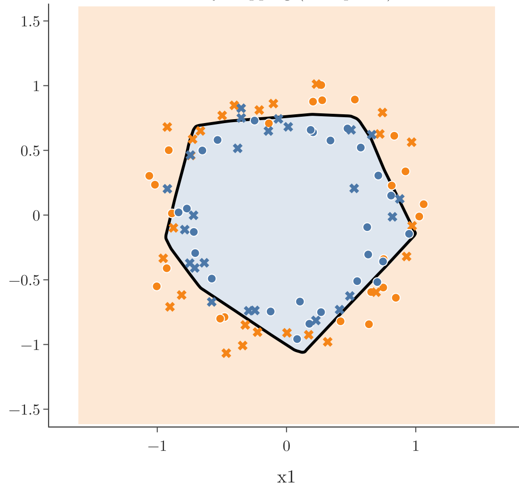
Early stopping (503 epochs)
