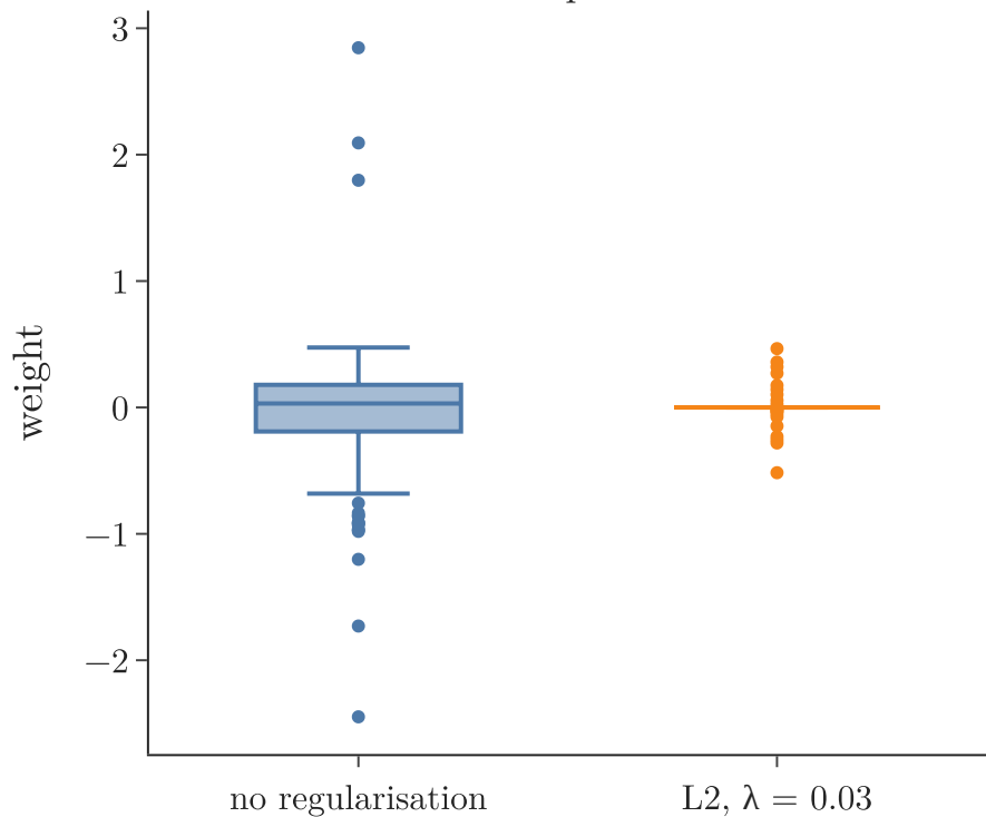
Box plots
