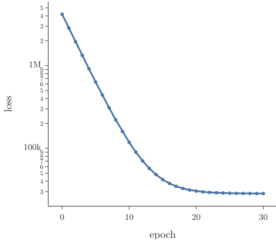
Loss after each epoch
