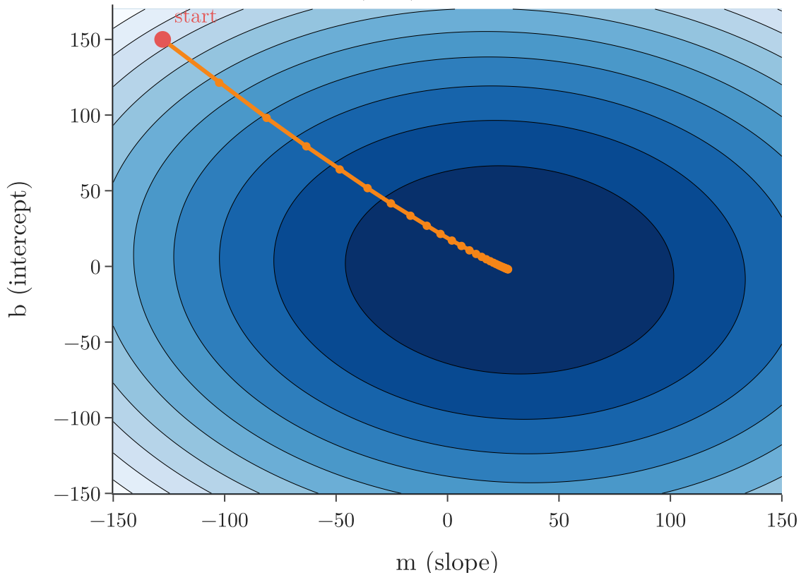
Path of (m, b) on the loss contours
