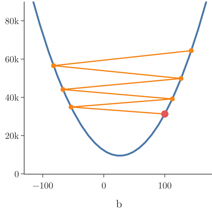
learning rate 0.26: overshoots, moves away
