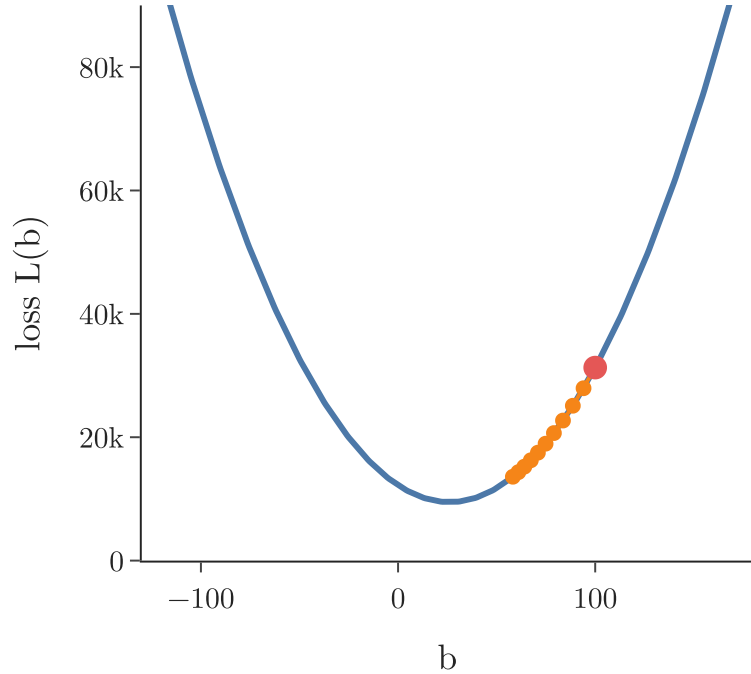
learning rate 0.01: tiny steps, 10 steps not enough
