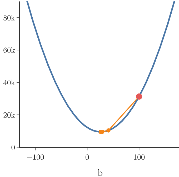
learning rate 0.1: reaches the bottom
