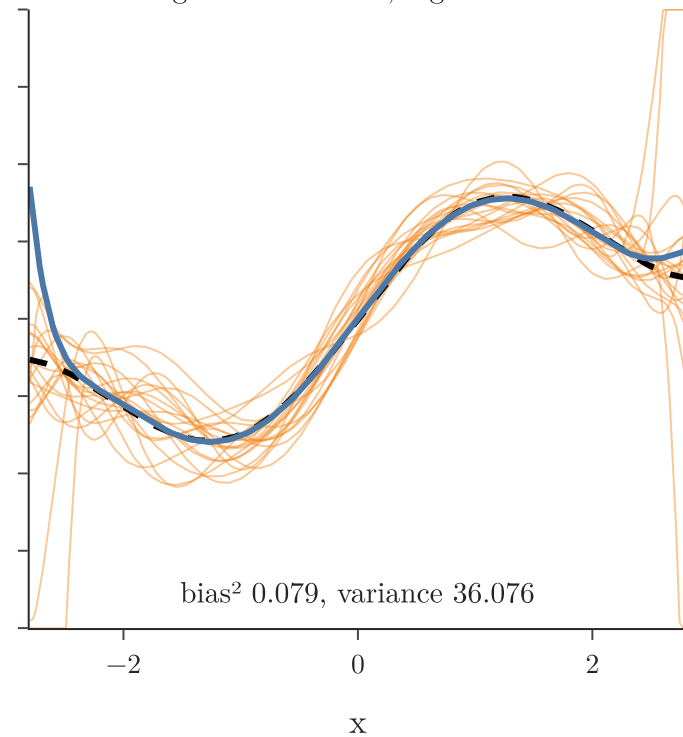
Degree 11: low bias, high variance
