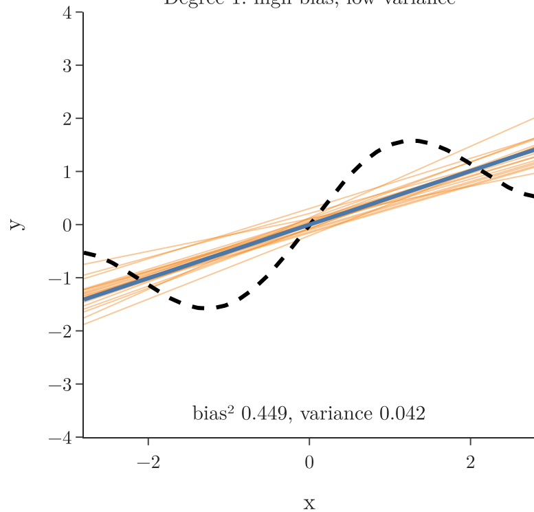
Degree 1: high bias, low variance
