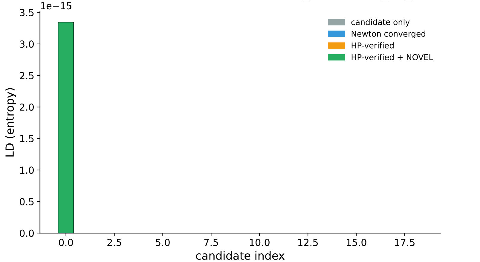
Candidates by LD, colored by survival status (n_total=19, n_HP_NOVEL=2)
