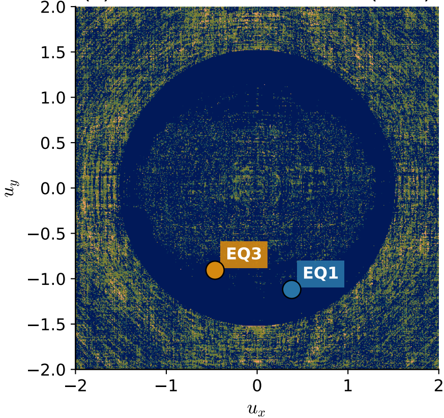
(c) HP-verified candidates (n=2)
