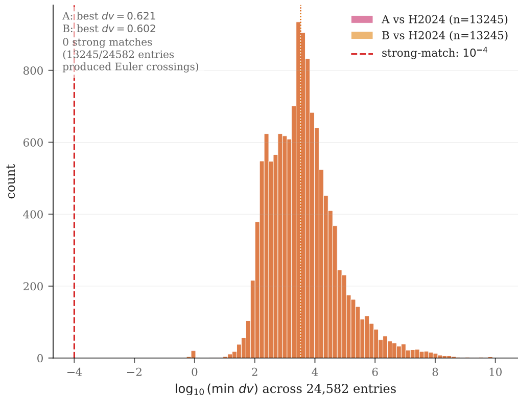
Panel 2 — min- dv distribution vs Hristov 2024 free-fall (24,582)
