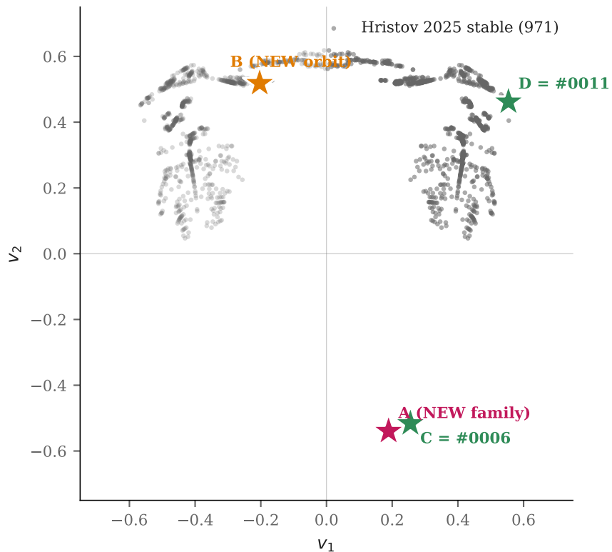
Panel 1 — against Hristov 2025 stable catalog (971 orbits)
