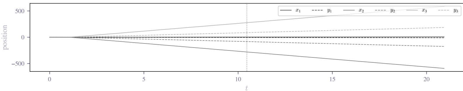
Position vs time
