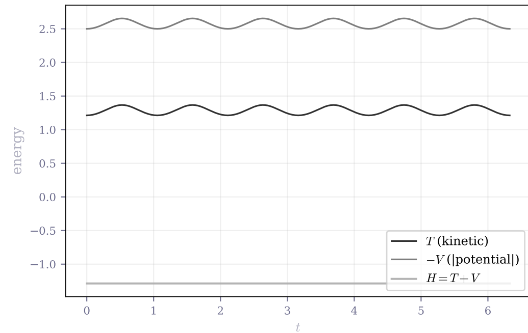
Figure-eight — virial ratio \langle T \rangle / (-\langle V \rangle / 2) = 1.0000
