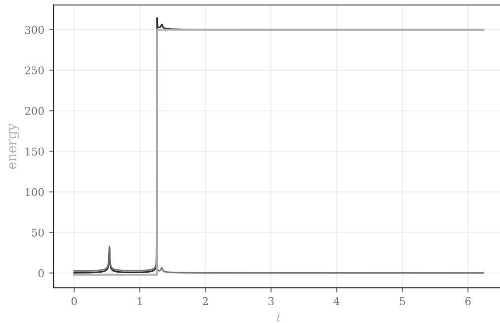
Butterfly I — virial ratio \langle T \rangle / (-\langle V \rangle / 2) = 474.9726
