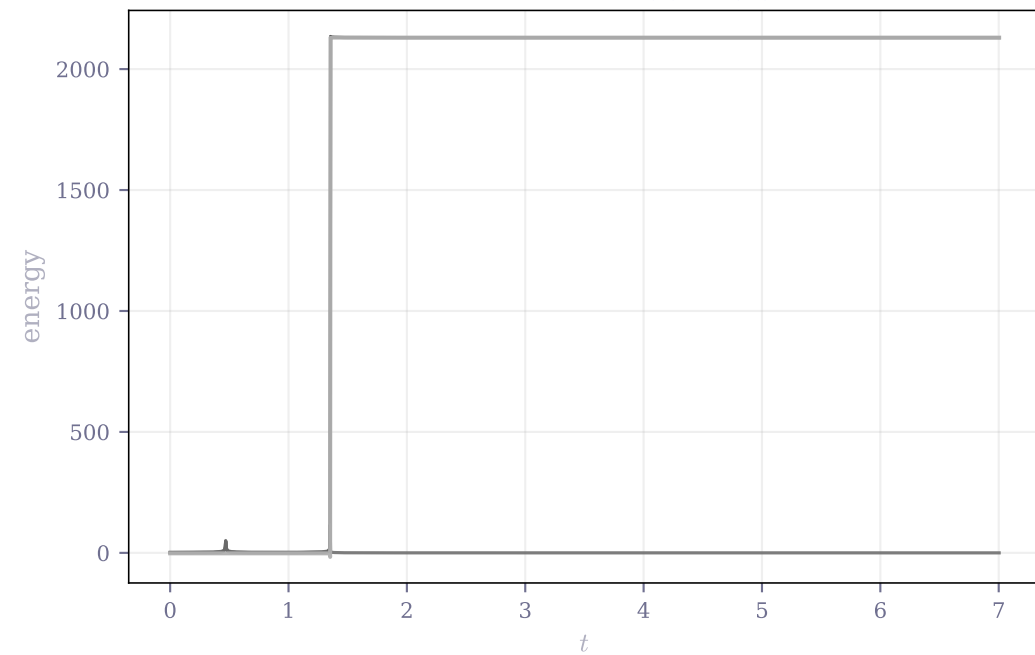
Butterfly II — virial ratio \langle T \rangle / (-\langle V \rangle / 2) = 4067.8305
