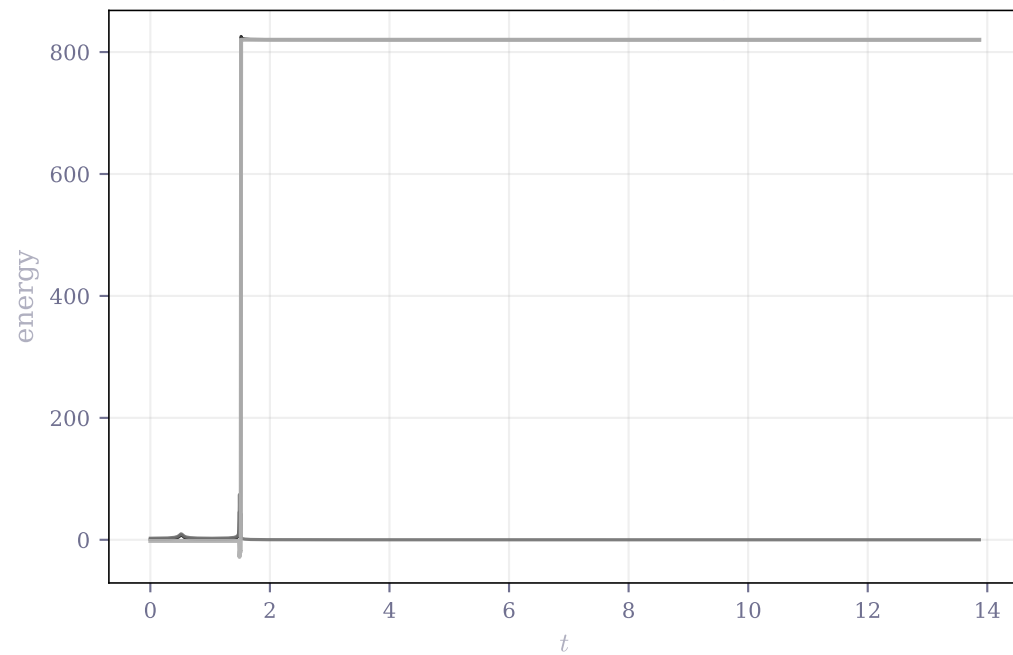
Butterfly III — virial ratio \langle T \rangle / (-\langle V \rangle / 2) = 2877.8172
