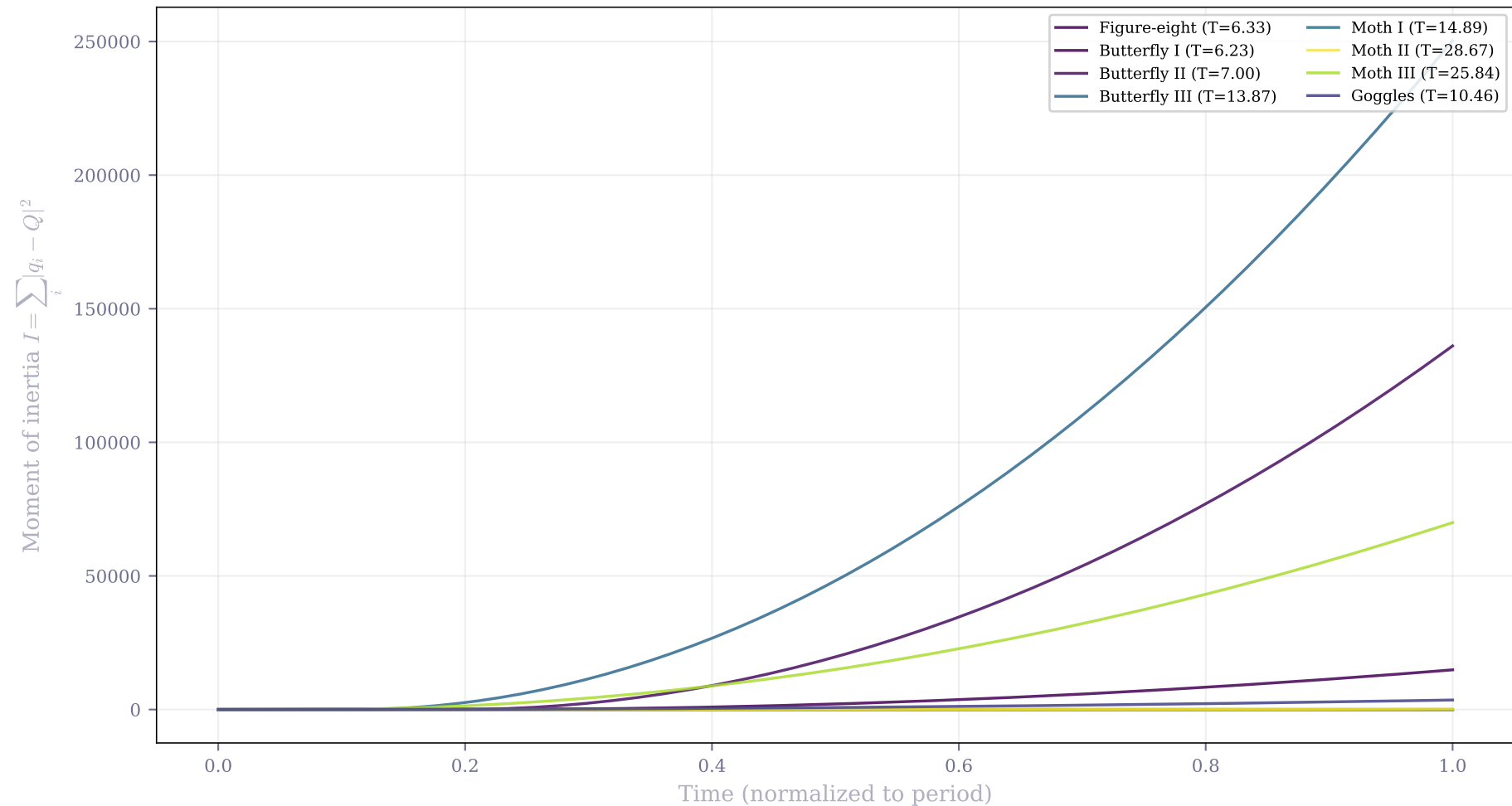
Breathing pattern: how compact the three-body system is All orbits start collinear ( I=2 ); expand and contract differently
