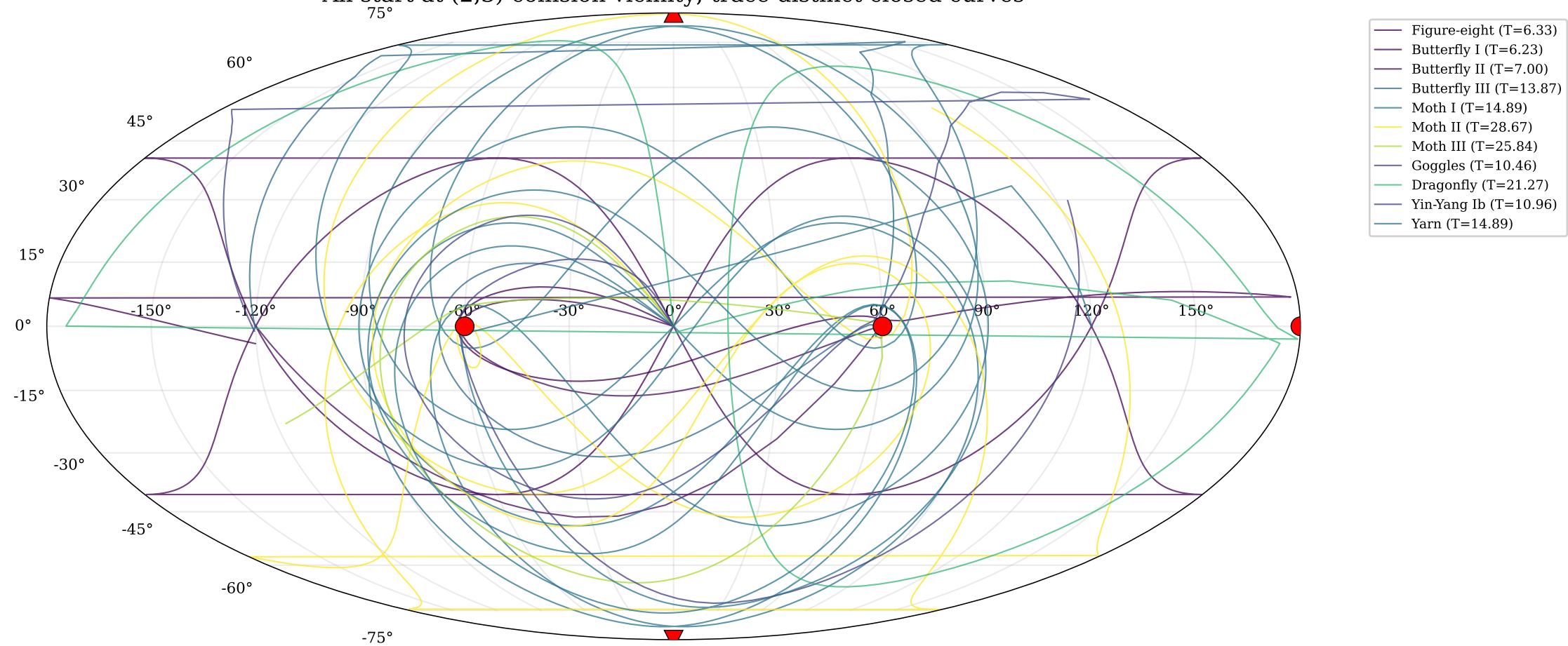
Shape-sphere paths of all 11 Suvakov orbits All start at (2,3)-collision vicinity; trace distinct closed curves
