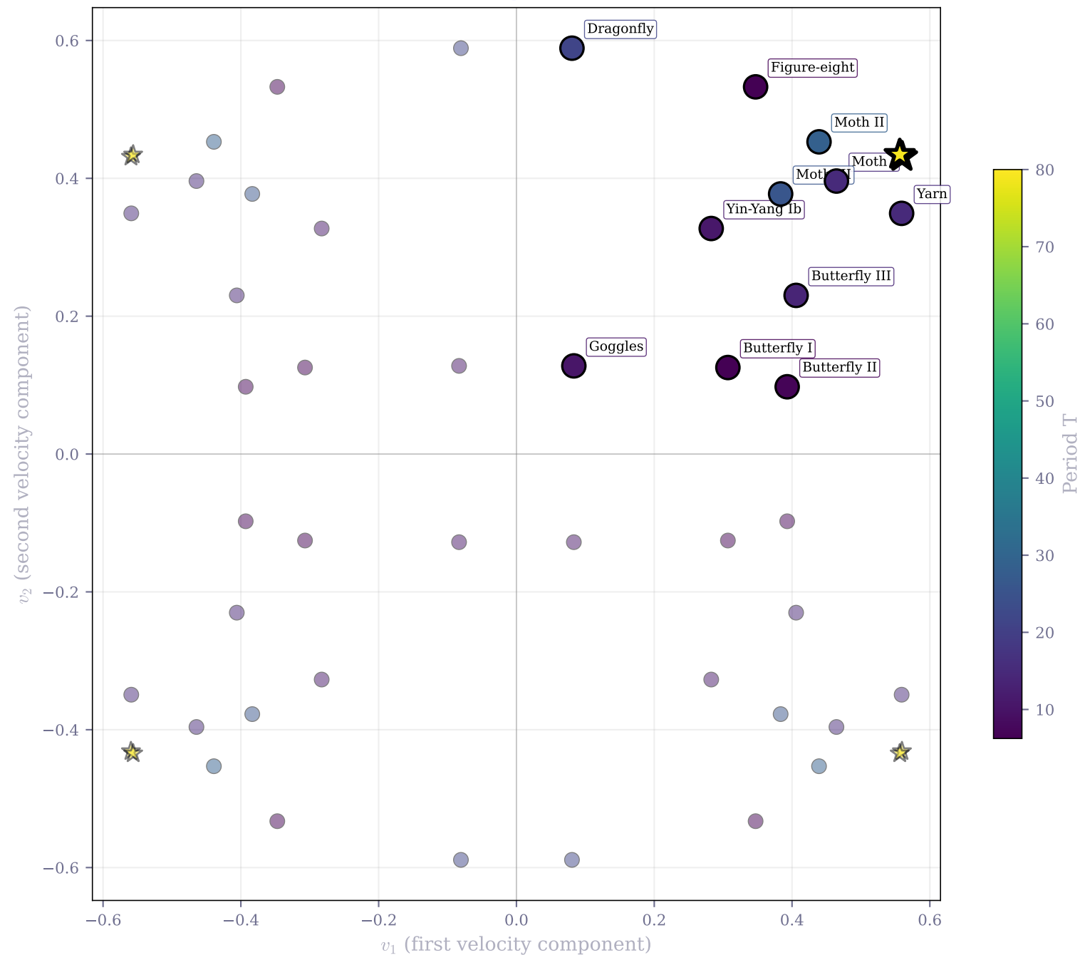
Periodic orbit constellation in velocity space Circles: Suvakov catalog. Stars: our discoveries.
