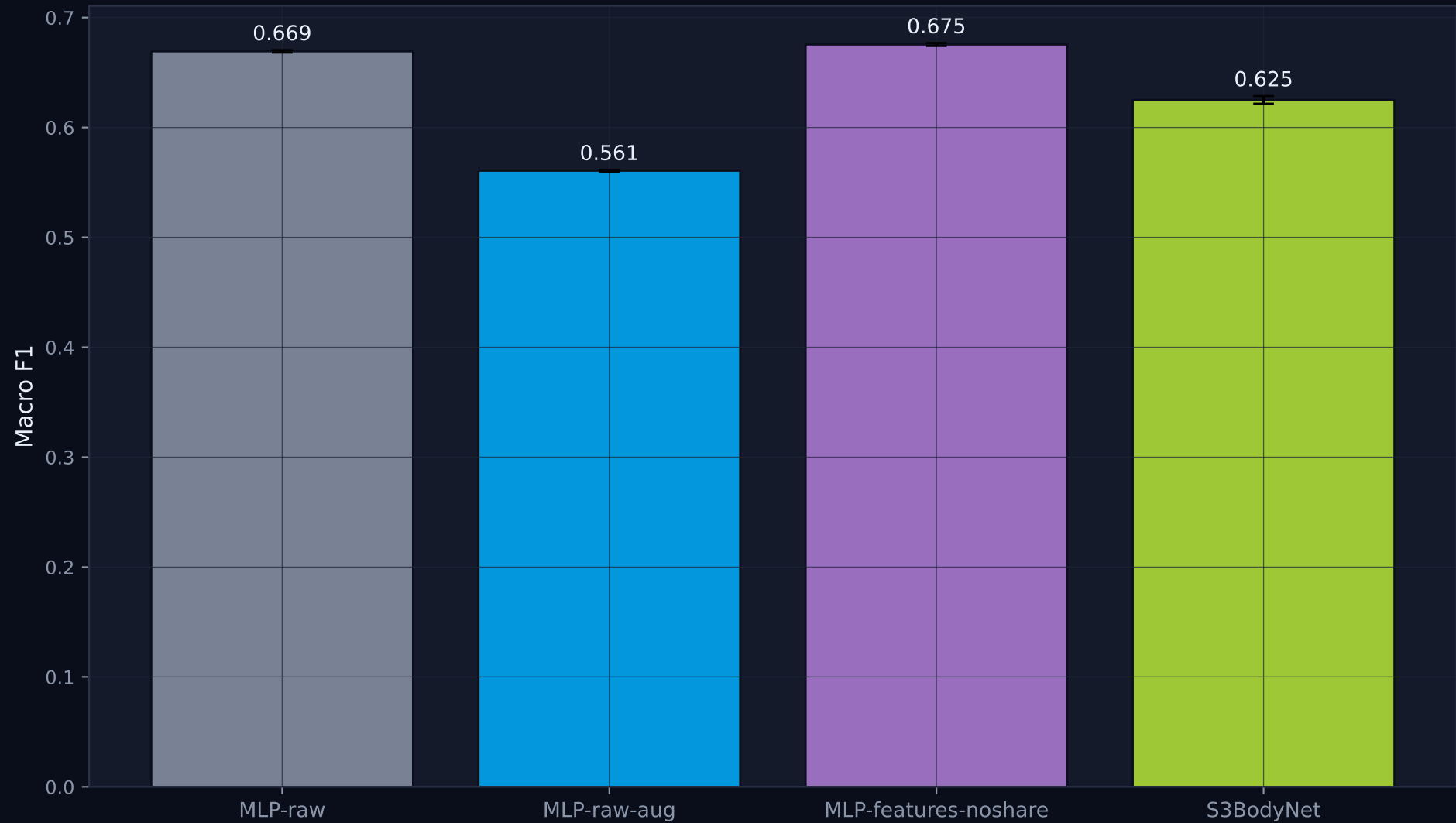
Four-way ablation (6D, N=300k, 5 seeds)
