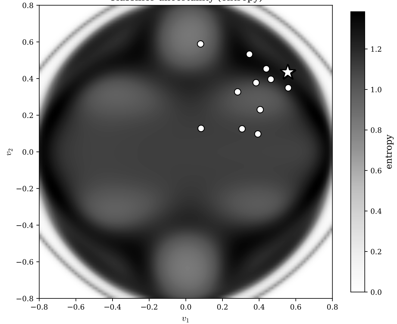
Classifier uncertainty (entropy)
