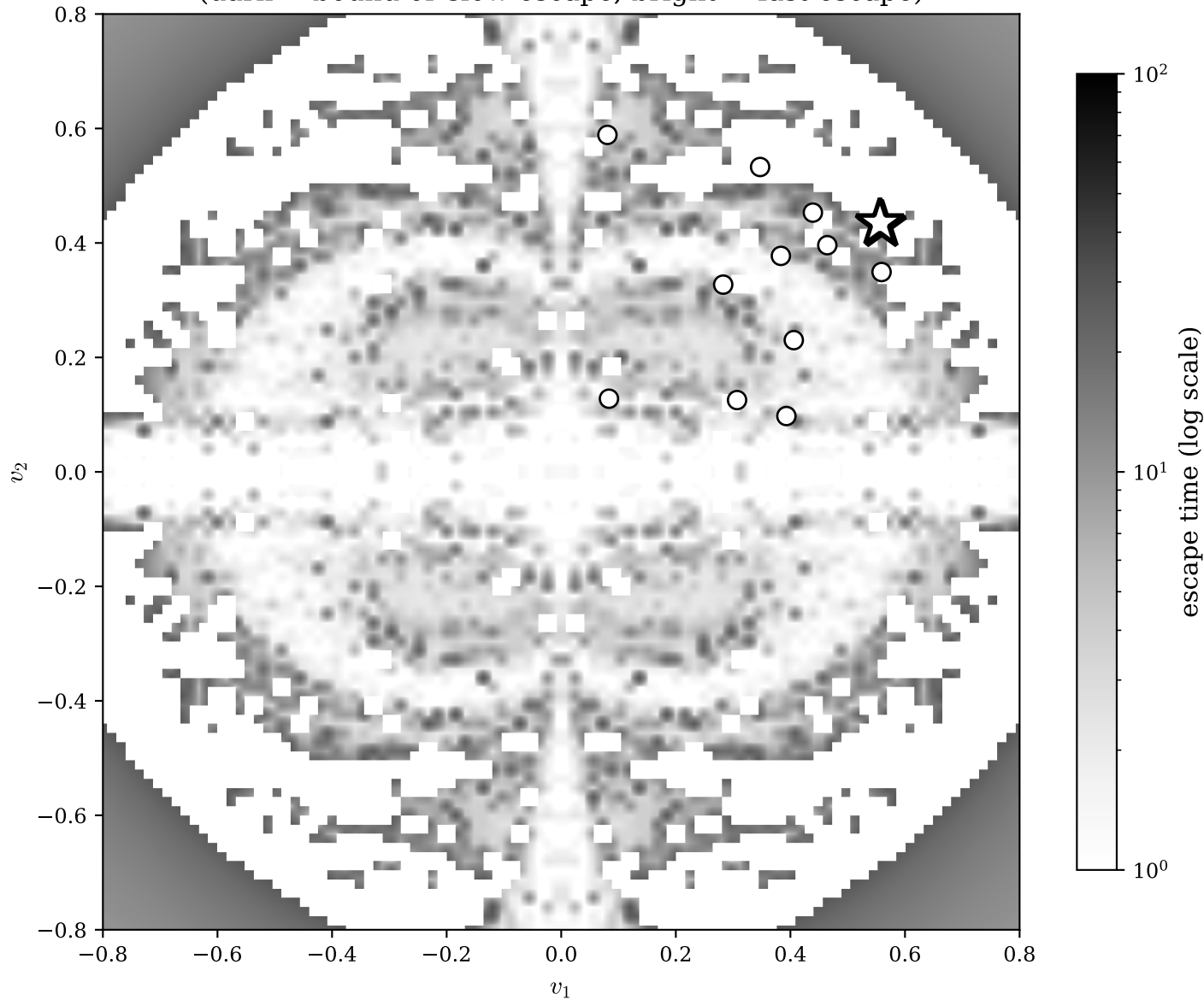
Escape time map (dark = bound or slow escape; bright = fast escape)
