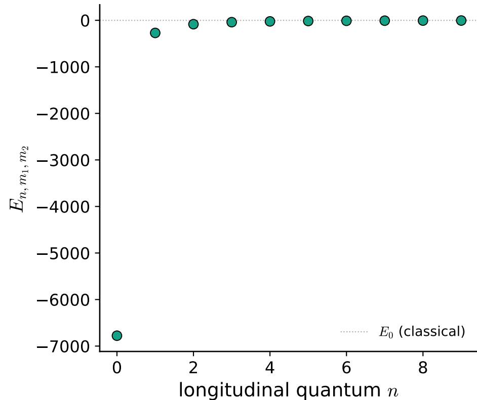
Orbit C (elliptic), \nu_{\text{mod } 2} = 1
