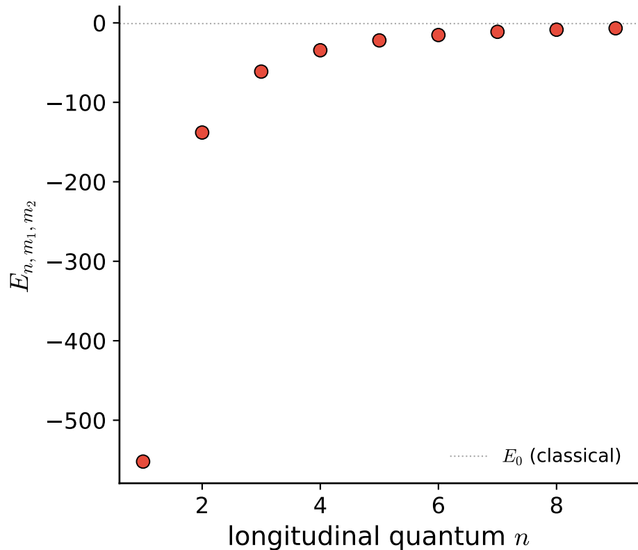
Orbit D (elliptic), \nu_{\text{mod } 2} = 0
