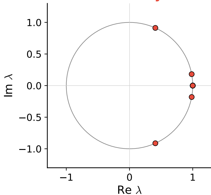
Orbit D: linearly stable
