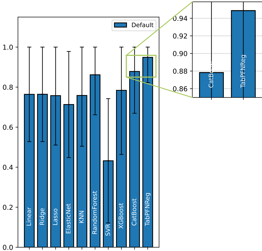
Normalized RMSE (normalized) (higher is better)
