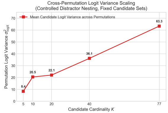
(b) Mean cross-permutation logit variance ( \sigma_{logit}^2 ).
