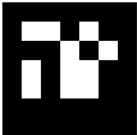
#11 C3_FLAME_TEST
