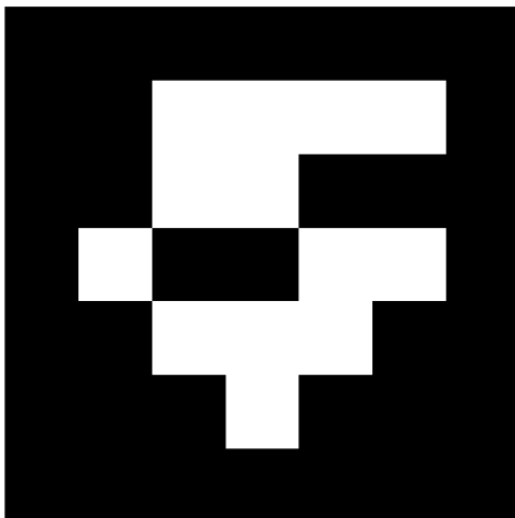
#18 C12_SERIES
