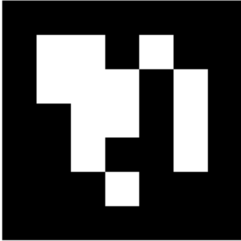
#4 P5_REFRACTION
