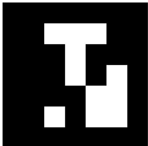
#7 P8_PHOTOELECTRIC
