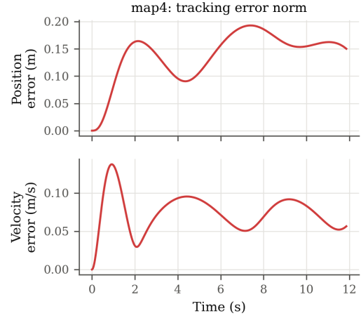
Fig. 4: Map 4 error vs. time. The error stays bounded within the safety region while maintaining performance.
