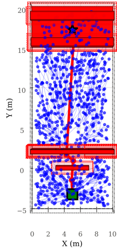
map1: RRT* tree with reduced path (top view)
