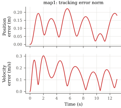
Fig. 3: Map 1 error vs. time. The error stays bounded within the safety region while maintaining performance.
