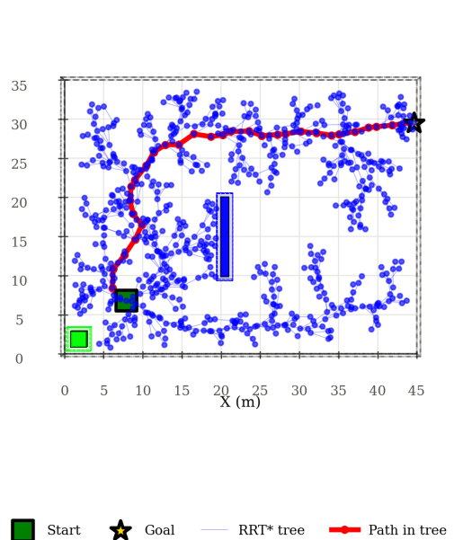
Fig. 2: Top-down view of the RRT* nodes expanded on Map 4.
