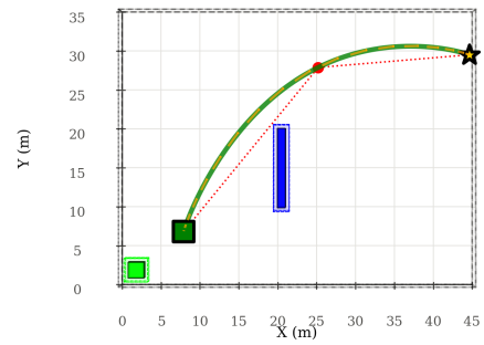
map4: spline trajectory, 13.6 s (top view)
