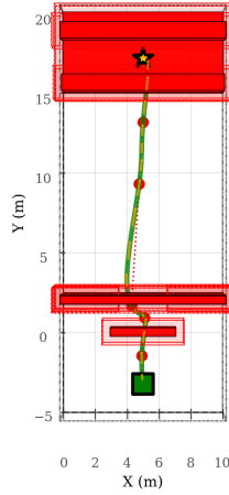
map1: spline trajectory, 14.0 s (top view)
