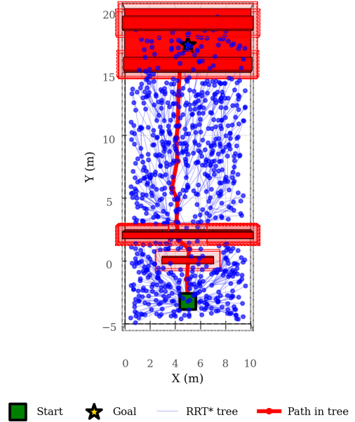
Fig. 1: Top-down view of the RRT* nodes expanded on Map 1.
