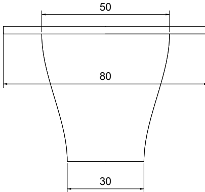
SIDE ELEVATION
