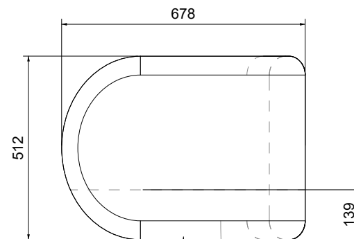
— REMOVE FOAM TILL 139MM AND REPLACE IT PLY TO CONNECT WITH THE CARCASS
