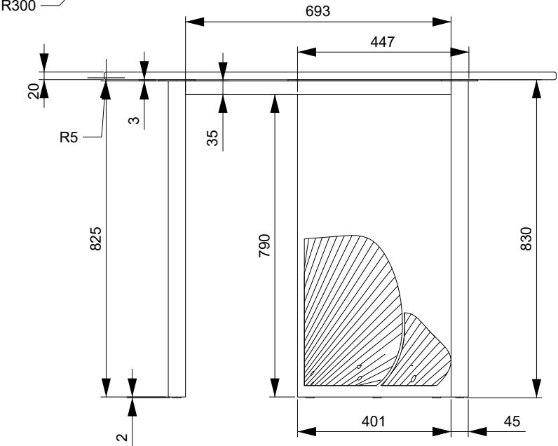
FRONT ELEVATION
