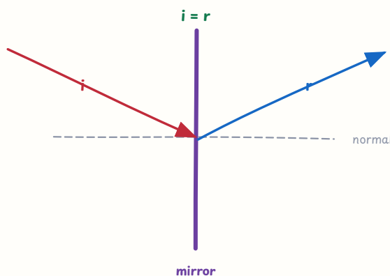
चित्र 7 — the incident and reflected rays make equal angles with the normal
