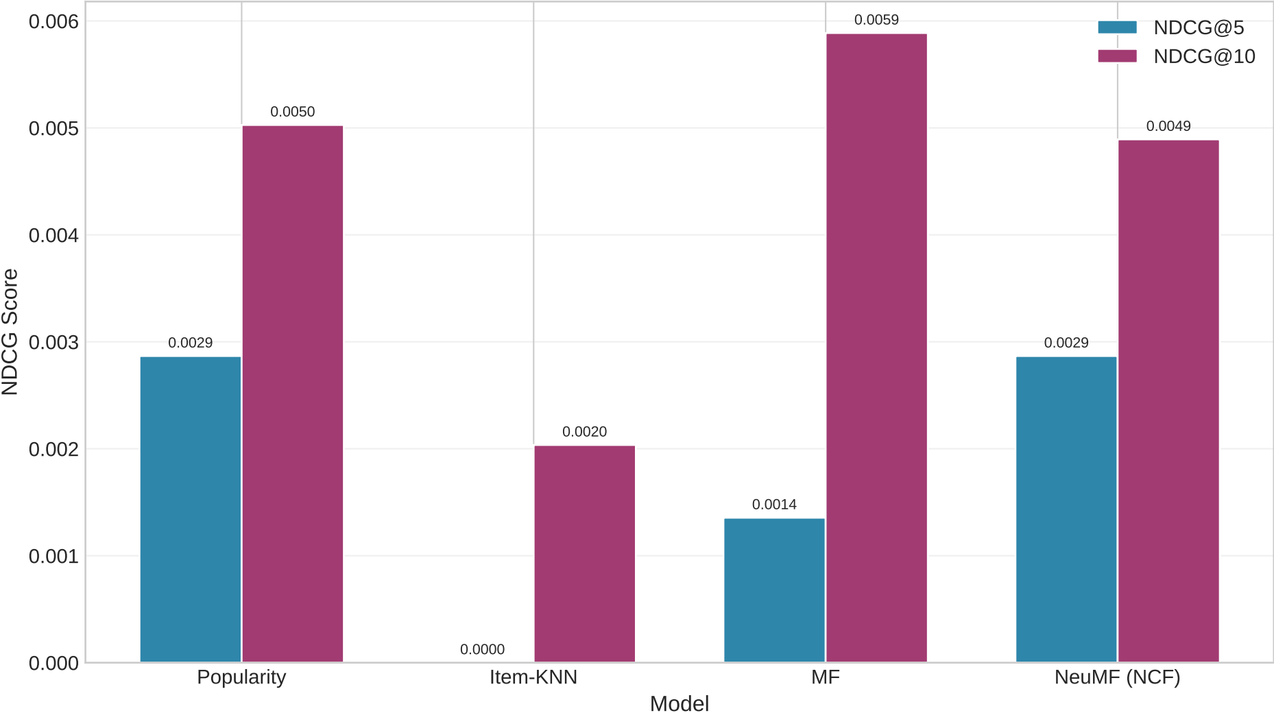
NDCG@K Comparison Across Models
