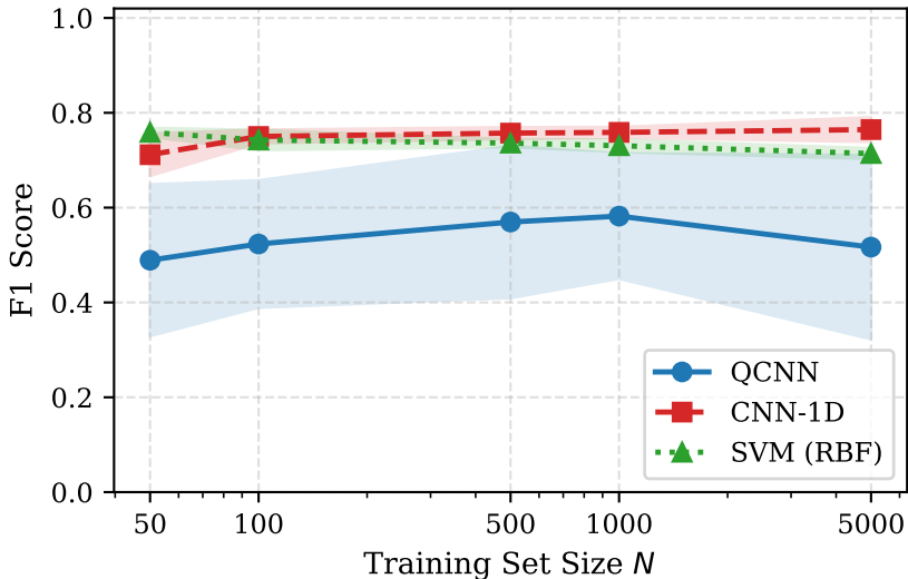
Data Efficiency on NSL-KDD (Binary Classification)
