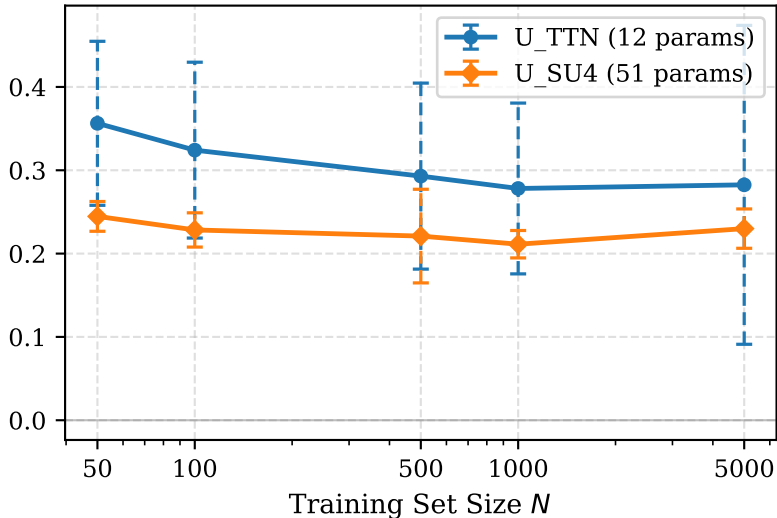
QCNN Generalization Gap vs. Training Size
