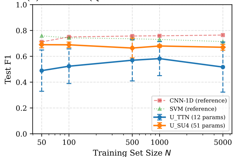
(a) Mean F1 (QCNN vs. classical reference)
