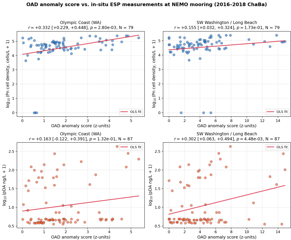
Figure 5. OAD anomaly score vs. in-situ ESP measurements at the NEMO mooring (47.97° N, 124.97° W) during the 2016–2018 ChaBa deployments. Top row: Pseudo-nitzschia cell density (sum of toxin-producing species via SHA assay, \log_{10} -transformed). Bottom row: particulate domoic acid via cELISA assay ( \log_{10} -transformed). Columns show the two regional OAD scores closest to NEMO. Reported Pearson r and 95% bootstrap CIs are computed on raw values (text uses raw correlations; plot uses \log_{10} axes for visual clarity). The strongest Pn correlation appears in the Olympic Coast region containing NEMO; the strongest pDA correlation appears in SW Washington, consistent with downwind transport of the toxin from the source.
