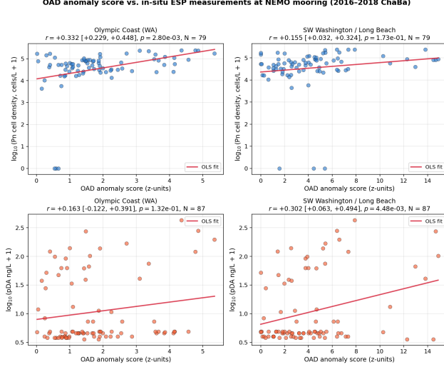
Figure 4. OAD score vs. ESP in-situ measurements at NEMO, 2016–2018. Top: Pn cell density ( \log_{10} ). Bottom: pDA ( \log_{10} ). Columns show the two regions closest to NEMO. Reported r and 95% CIs use raw values; log-axes shown for visual clarity only.
