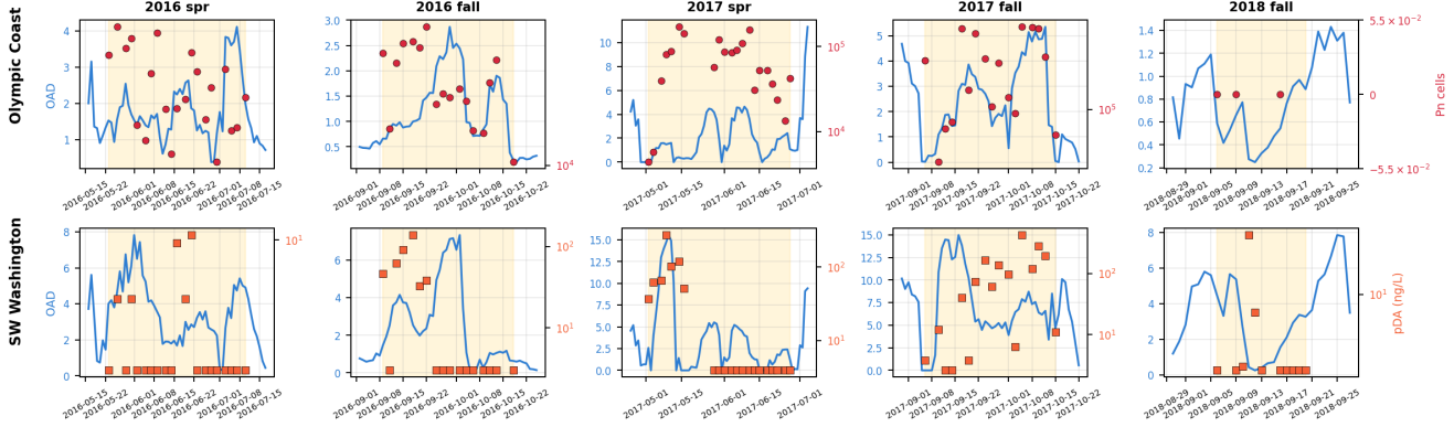
Figure 5. Time-series overlay of OAD anomaly score (blue line, left axis) and ESP in-situ measurements (markers, right axis on symlog scale) across the five 2016–2018 ChaBa deployment windows (yellow shading \pm 7 days of context). Top row: Olympic Coast OAD vs. ESP Pn cell density. Bottom row: SW Washington OAD vs. ESP pDA. The temporal co-evolution of the unsupervised satellite signal and the independent in-situ biology is direct visual confirmation that OAD captures real bloom dynamics at the source. The 2017 spring deployment (third column) is particularly informative: the OAD score rises noticeably before the ESP-measured Pn spike.
