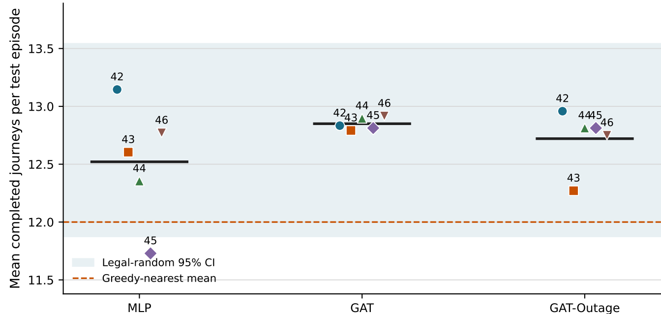
Clean-test completed journeys by trained policy
