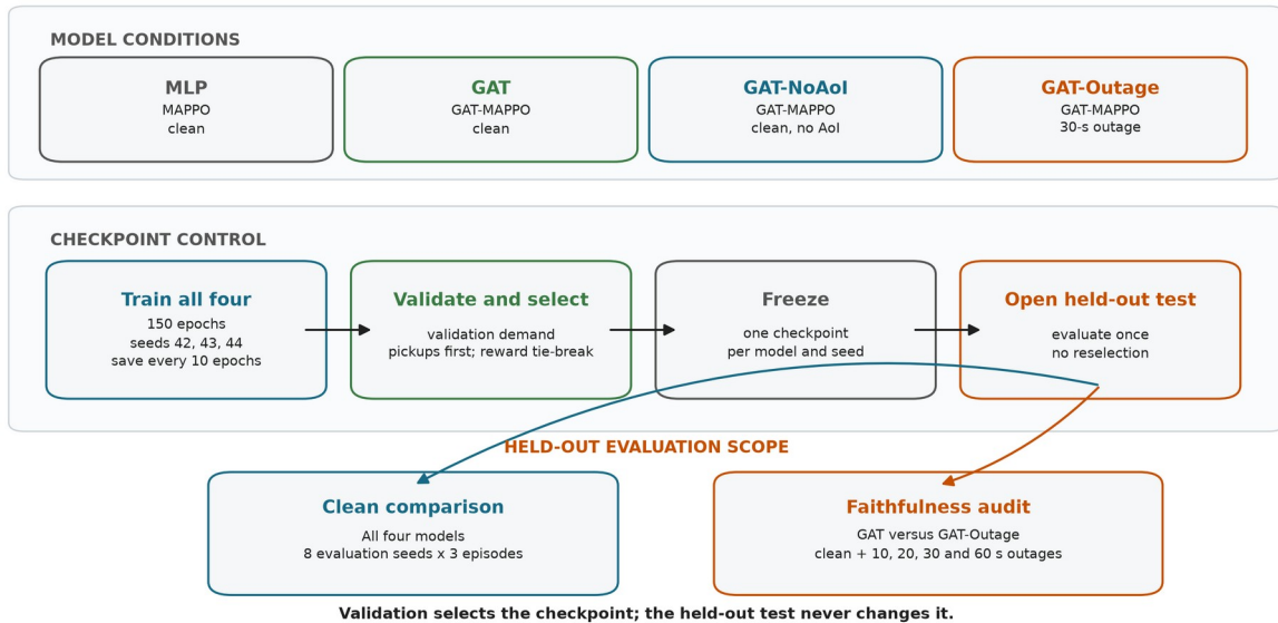
Figure 3.3. Common training and validation-based checkpoint selection for all four model conditions. Frozen checkpoints are evaluated on held-out demand; the faithfulness audit compares GAT and GAT-Outage.
