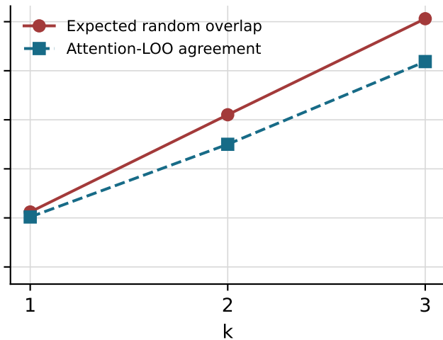
GAT-Outage
