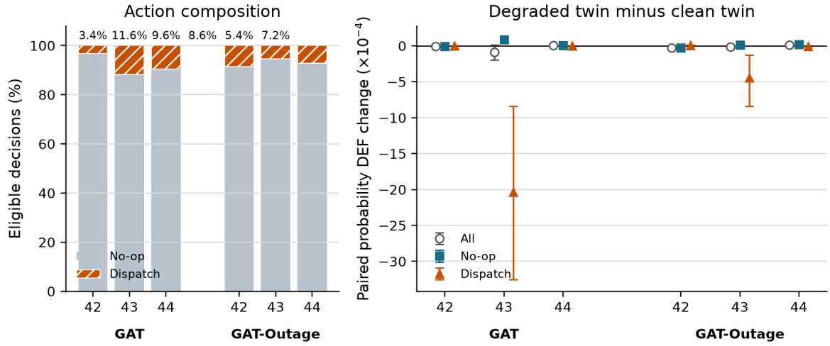
Figure 4.9. Left: eligible action composition for each checkpoint. Right: paired degraded-minus-clean probability DEF for all eligible decisions, chosen no-op actions, and dispatch actions. Error bars are 95% episode-block bootstrap intervals.
