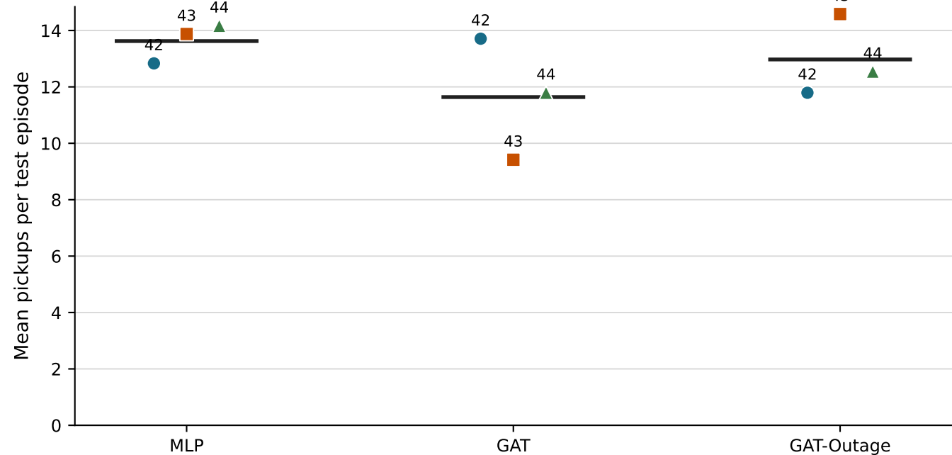
Clean-test pickups by trained policy
