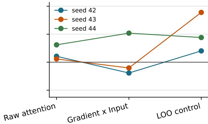
GAT-Outage
