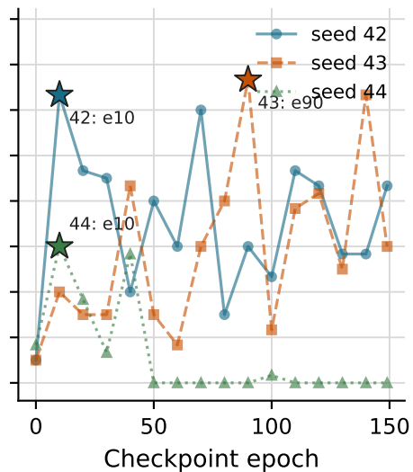
GAT-Outage
