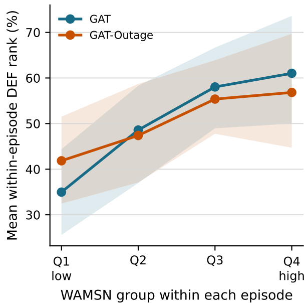
(a) DEF rank across WAMSN groups
