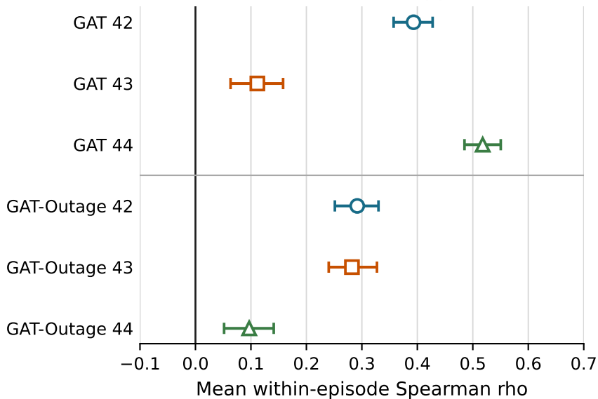
(b) H4 result: 0/6 supported
