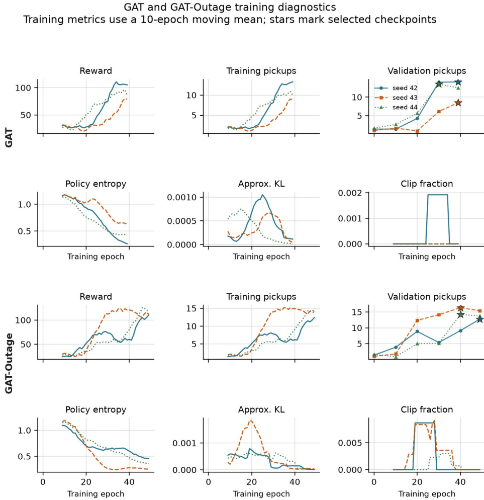
Figure 4.1. Training diagnostics for GAT (upper panels) and GAT-Outage (lower panels). Curves use a ten-epoch moving mean; stars mark validation-selected checkpoints. Entropy remains above the collapse threshold, and PPO clipping is limited.
