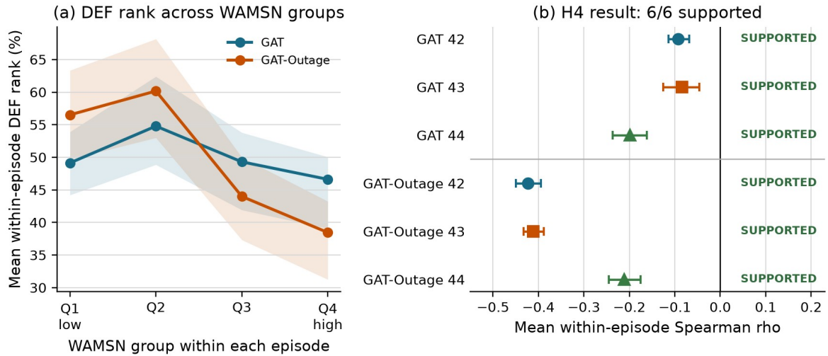
Figure 4.11. Panel (a) divides each usable episode into four equal-count WAMSN groups and plots the corresponding mean DEF rank. Q4 is lower than Q1 for both models, although the intermediate groups are not monotonic. Lines summarize episode blocks within each model, and shaded bands show their interquartile range. Panel (b) reports mean rho and a 95% episode-block bootstrap interval. Every checkpoint supports the fourth hypothesis after Holm correction.
