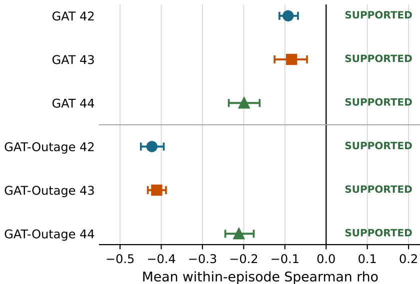
(b) H4 result: 6/6 supported
