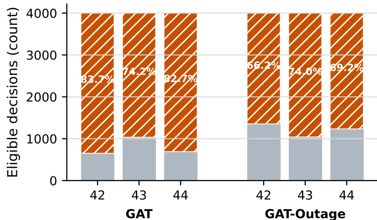
(a) Chosen-action counts
