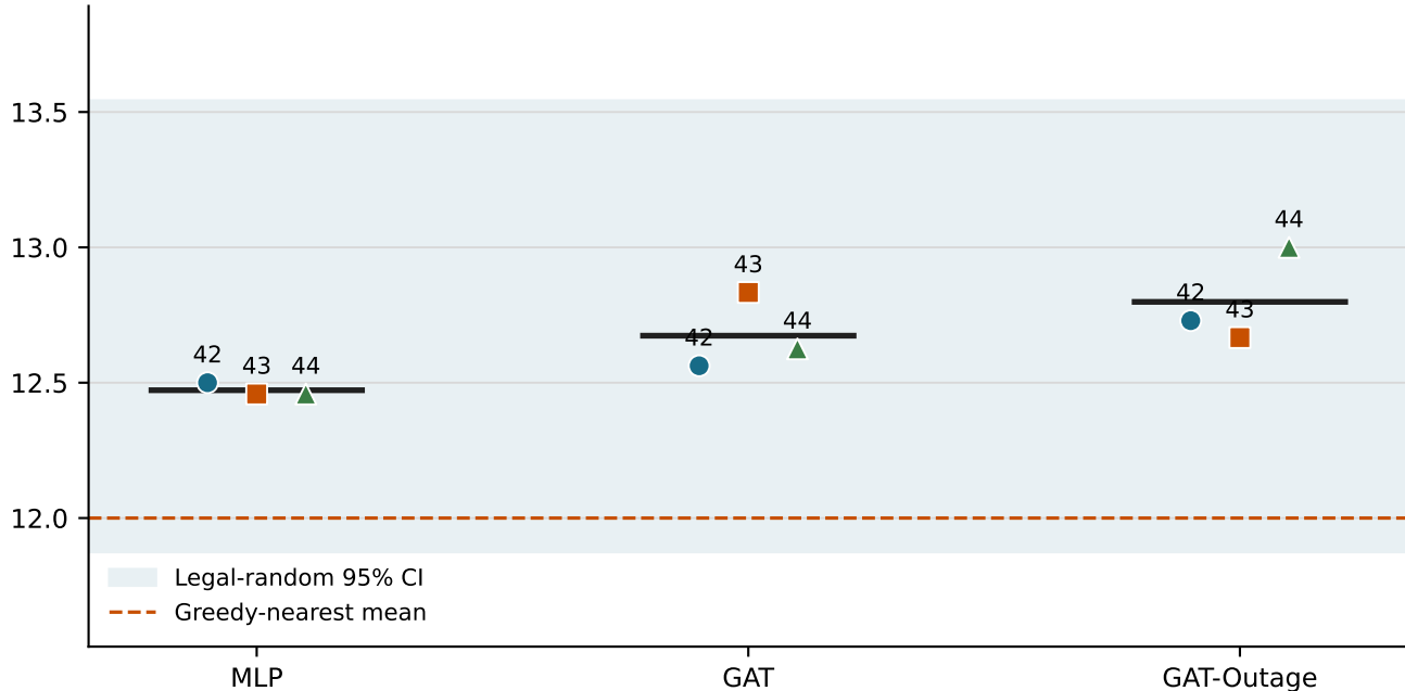
Clean-test completed journeys by trained policy
