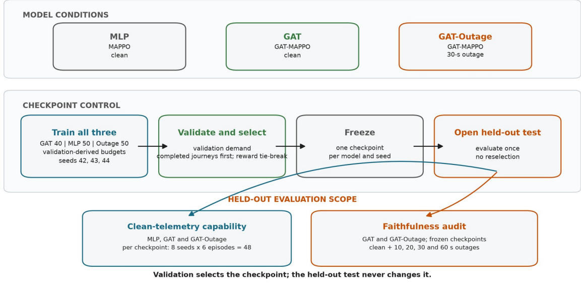
Figure 3.5. Shared training and validation-based selection pipeline with the model-specific budgets described above. Each frozen checkpoint receives 48 clean held-out episodes. The faithfulness audit then compares the frozen GAT and GAT-Outage checkpoints across clean and four outage conditions without reselection. This produces 720 faithfulness-sweep episodes per GAT model and 1,440 in total.
