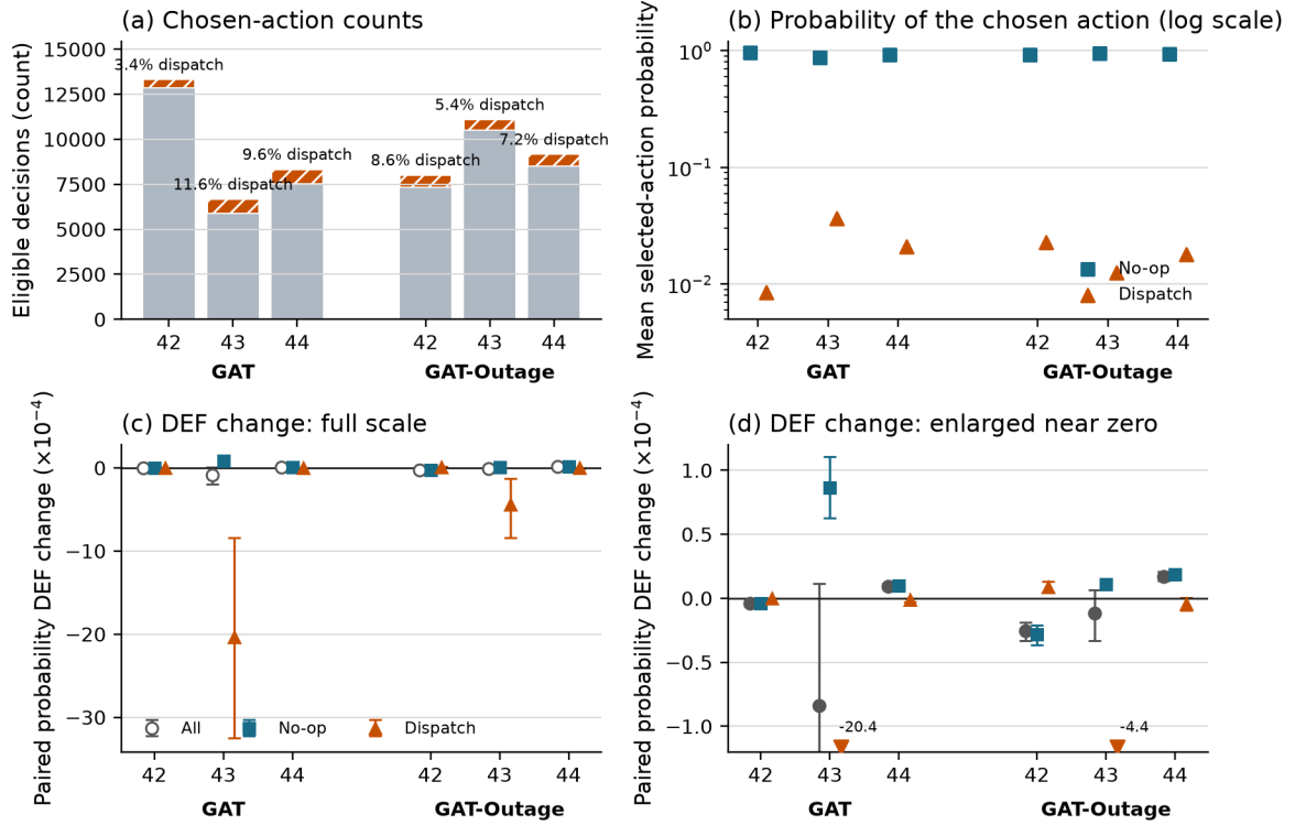
Figure 4.9. (a) Absolute no-op and dispatch counts; labels give the dispatch share. (b) Mean probability assigned to the sampled action on a logarithmic scale. (c) Paired degraded-minus-clean probability DEF on the full scale. (d) Enlarged view around zero; arrows mark intervals that extend beyond the panel. Error bars are 95% episode-block bootstrap intervals.
