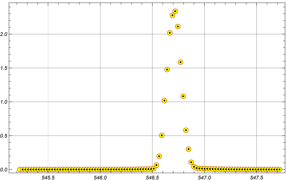
06_Hg_calibration_546.475nm_546.226_at_50_nm_hg_2nm_scan_REAL_FOR_CURVEFIT
