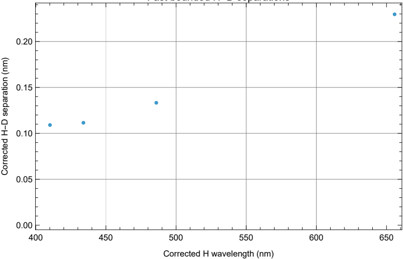
Fast bounded H-D separations
