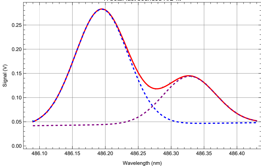
H beta: fast bounded H/D fit
