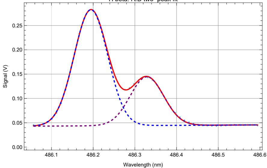
H beta: H/D two-peak fit
